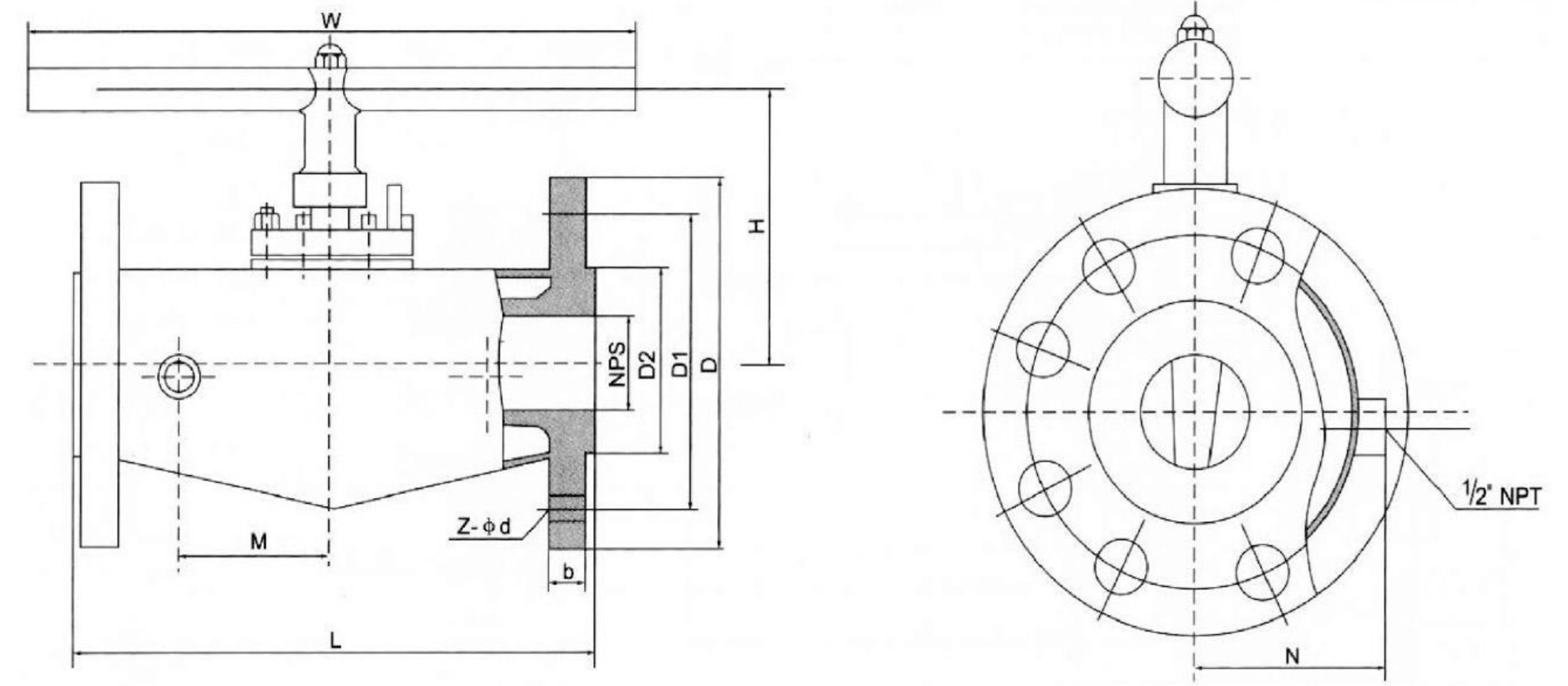
Main External and Connection Dimension
