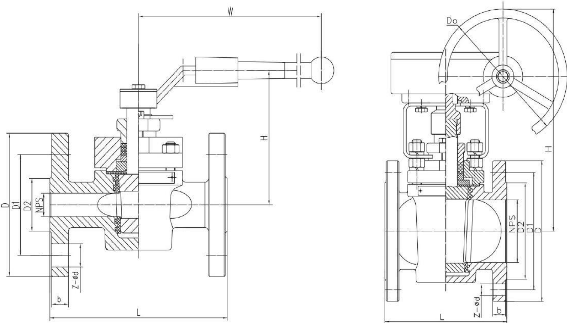
Main External and Connection Dimension
