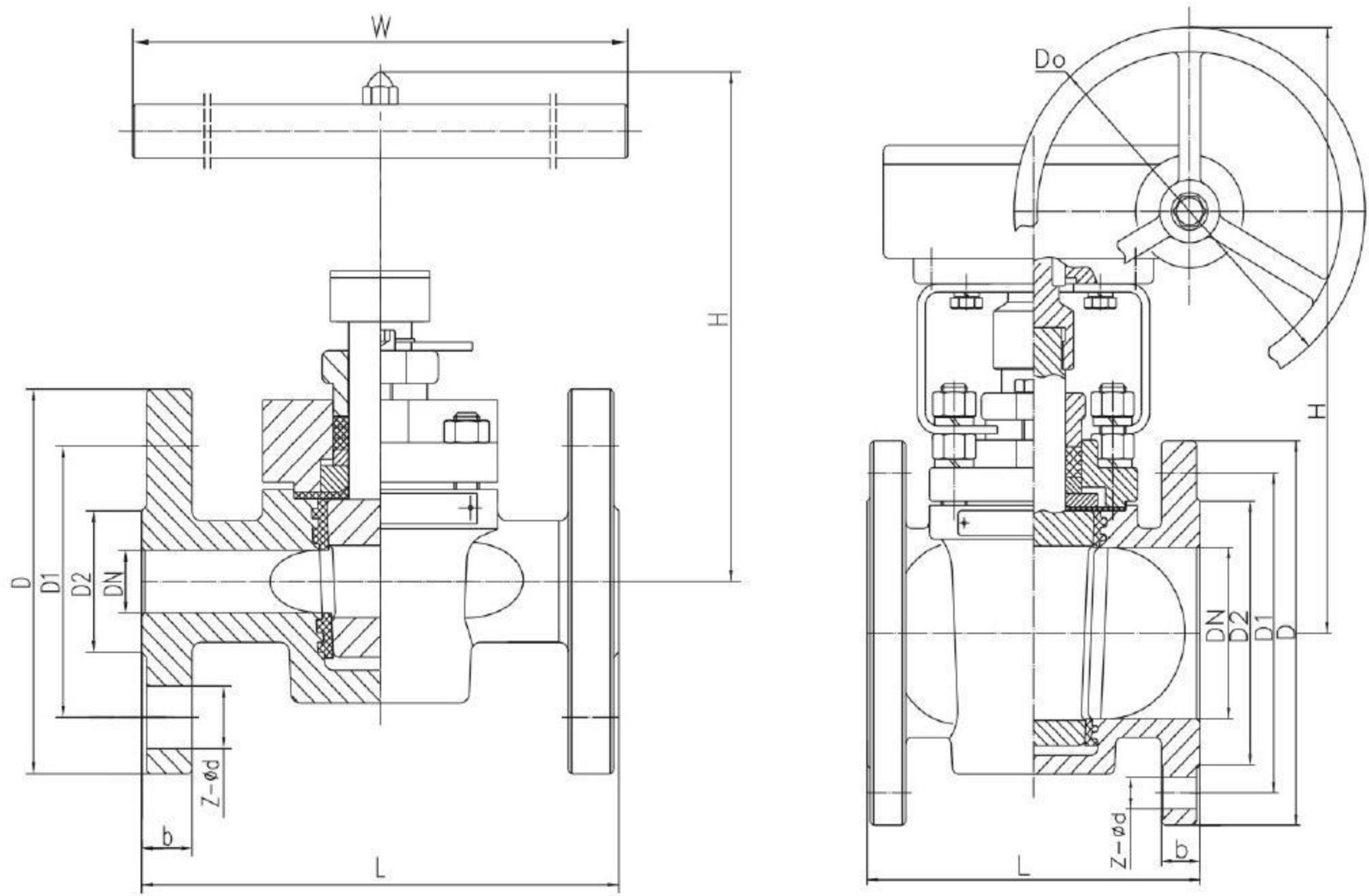
Main External and Connection Dimension
