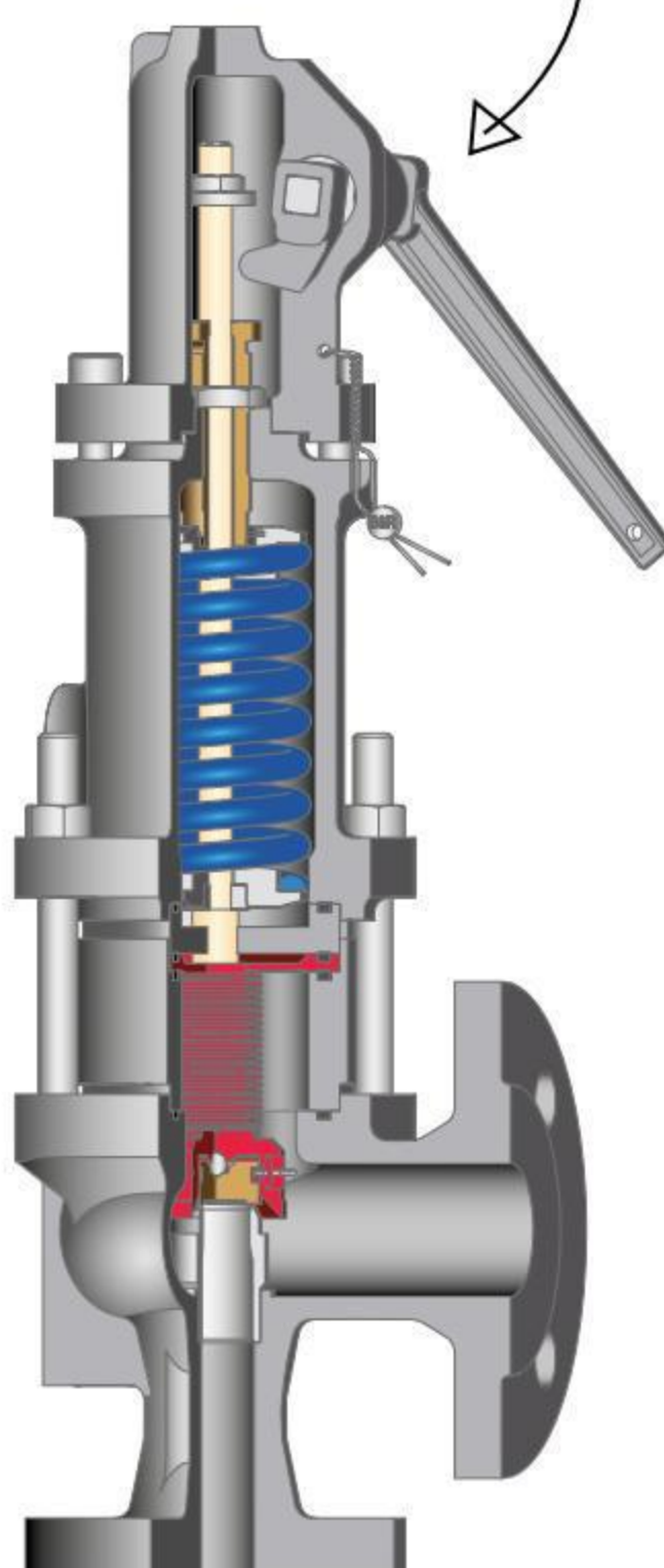
Safety valve with bellows
