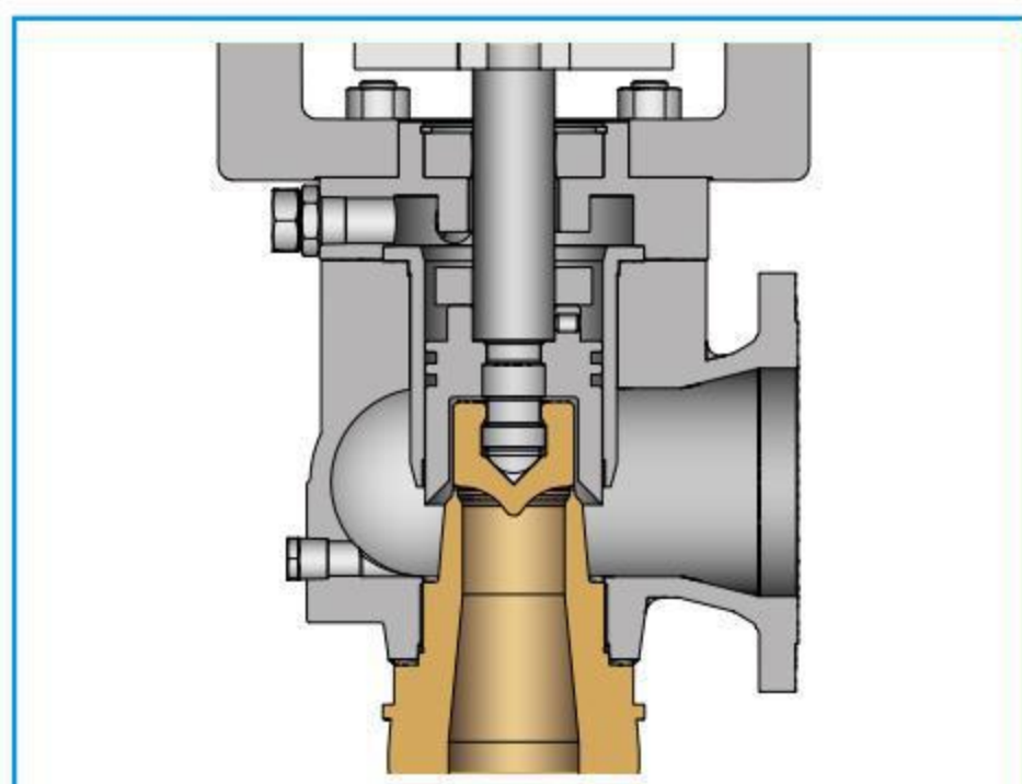
.22a Weld end at inlet.
