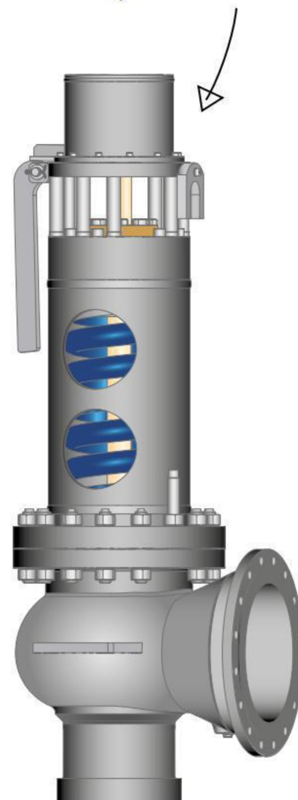
Safety valve with open bonnet
