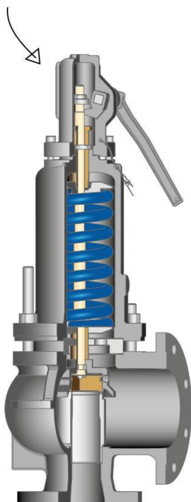
Conventional safety valve
